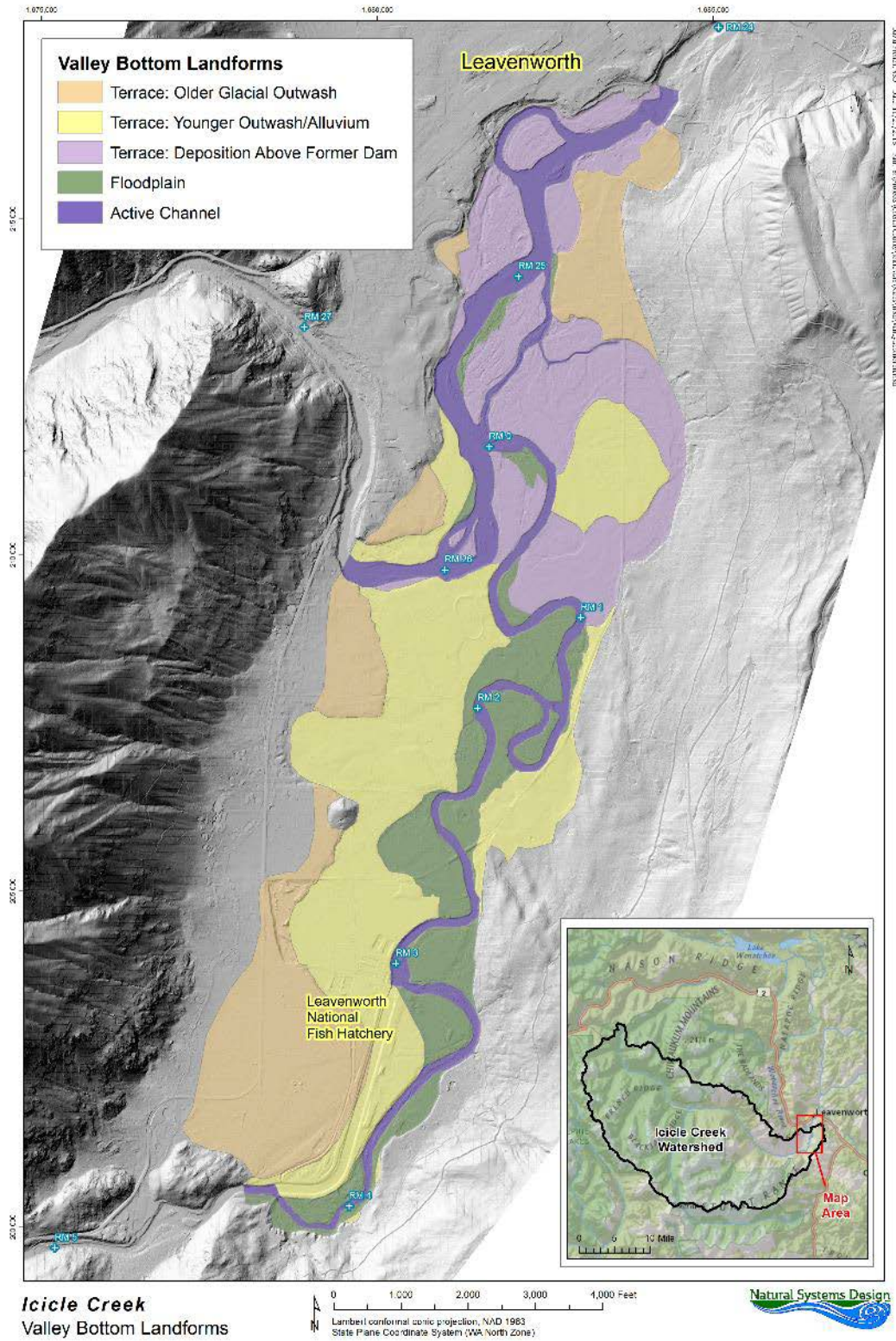
Figure 7. Geomorphologic map of the Lower Icicle Creek Valley.
