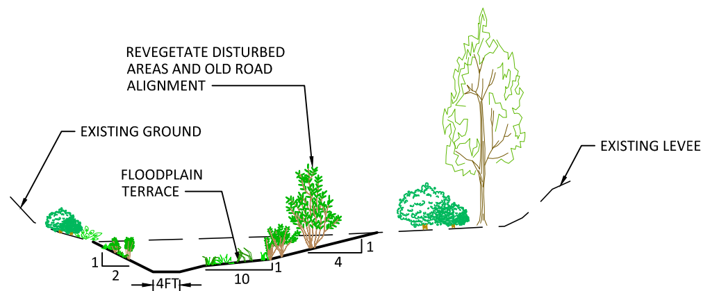
3 10 TYPICAL SECTION - CHANNEL REMEANDER NOT TO SCALE
