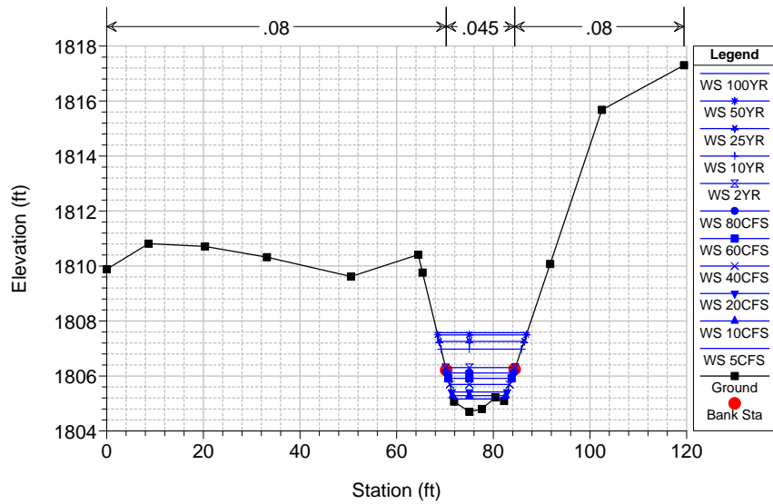
SkinnyCreekRM0-0.5 Plan: Skinny Creek - existing conditions 5/31/2016
