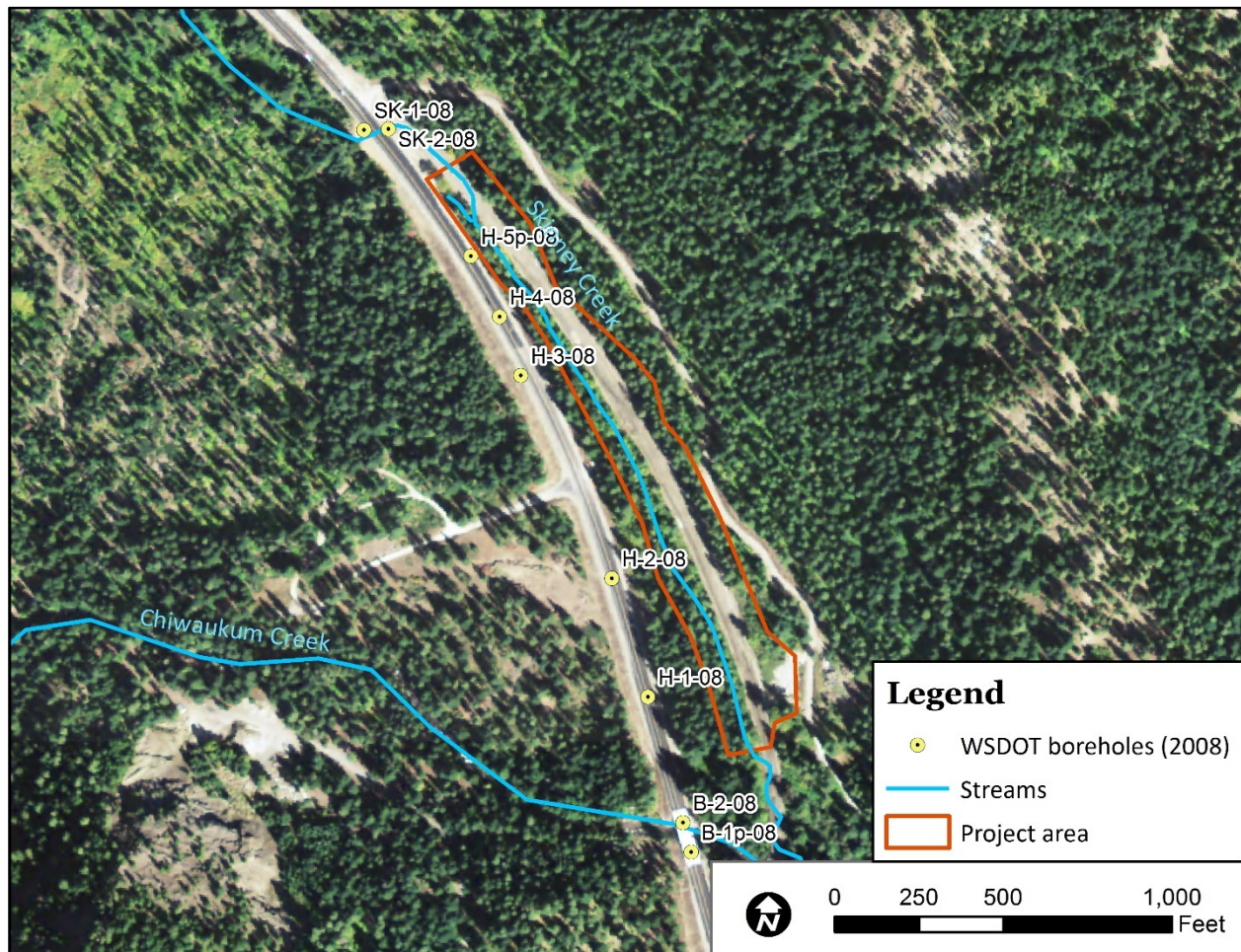
Figure 2. Locations of 2008 WSDOT boreholes.
