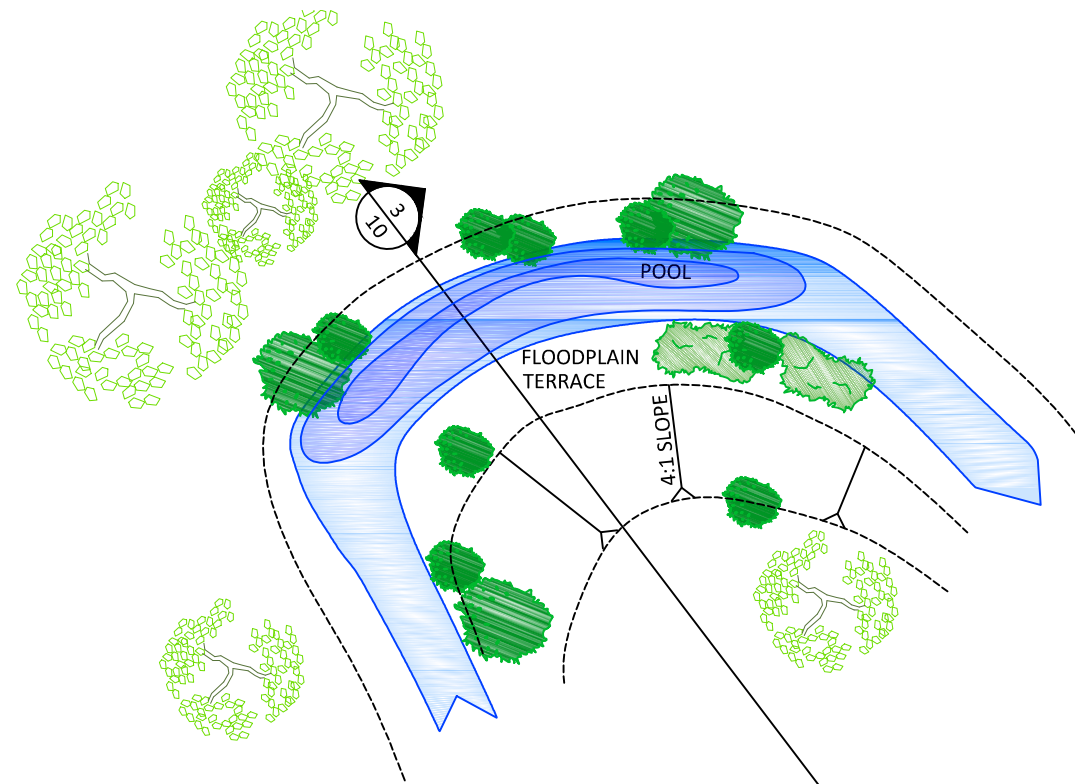
1 10 TYPICAL PLAN VIEW - INSET FLOODPLAIN NOT TO SCALE
