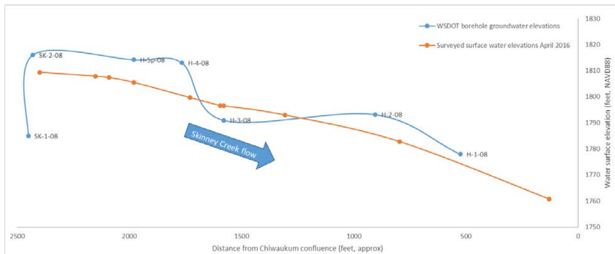
Figure 3. Groundwater elevations from 2008 boreholes plotted with surface water elevations surveyed in April 2016. The x-axis values are based on distance from Chiwaukum Creek on an arbitrary line drawn up the Skinny Creek Valley between the boreholes and surveyed water surface elevations.
