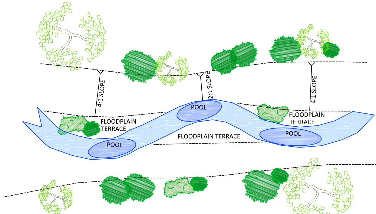
2 10 TYPICAL BANK GRADING NOT TO SCALE
