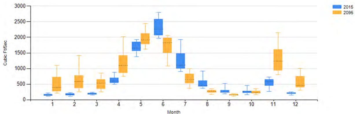
Figure 5. Boxplot of modeled average monthly flows at USGS gage 12447383 (Methow River above Goat Creek near Mazama, WA) for existing (2015) and future (2095) climate scenarios generated from Voss and Mastin (2012) web-based tool ( http://wa.water.usgs.gov/projects/methow/cc.htm ). Boxplots represent modeled values for all general circulation models and greenhouse gas emission scenarios. The boxes represent the semi-quartile range (25 to 75 percentile); dashed line is the median; and vertical lines extent to minimum and maximum values.
