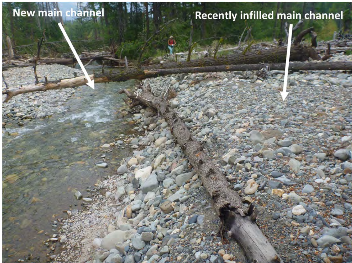
Figure 116. Change in channel location through infilling (instigated by wood accumulations during high flow) and avulsion at RM 75.75.
