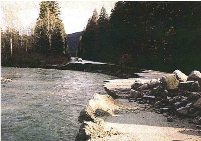
CED site #1: 1995 flood that washed out the SR 207 road prism near RM 4.5. Photo taken from the south looking north.
